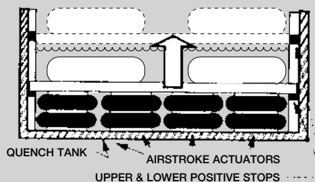
QUENCH TANK ACTUATOR
