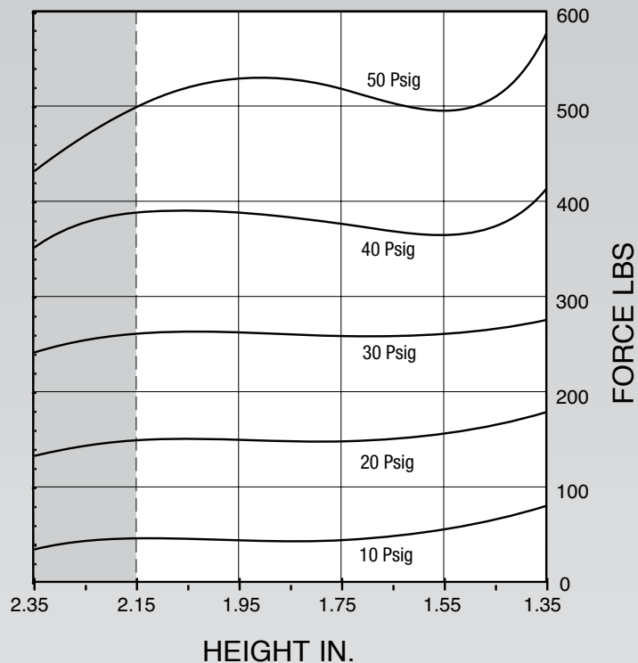
Force Table (Use for Airstroke™ actuator design)
