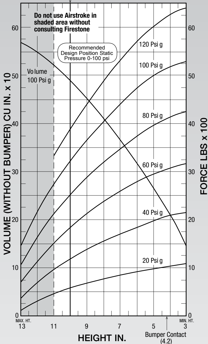
Force Table (Use for Airstroke™ actuator design)
