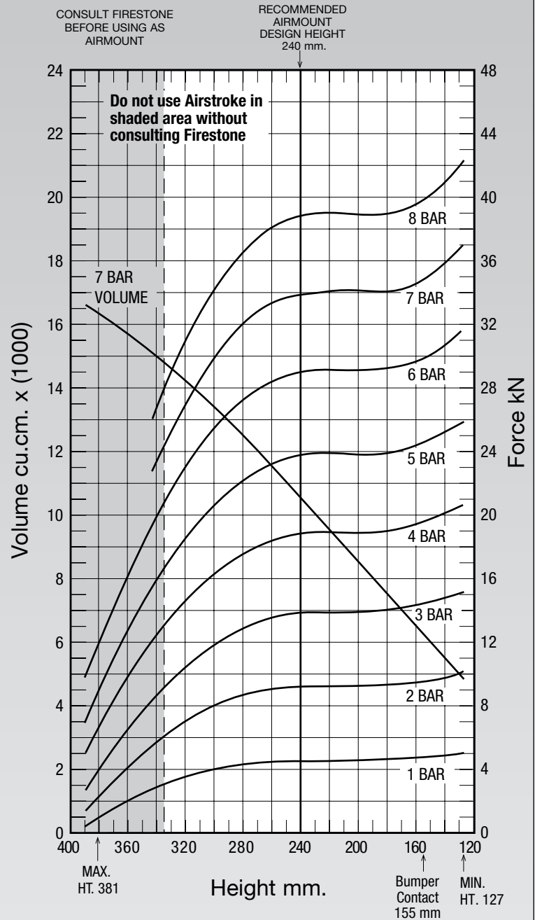
Force Table (Use for Airstroke™ actuator design)
